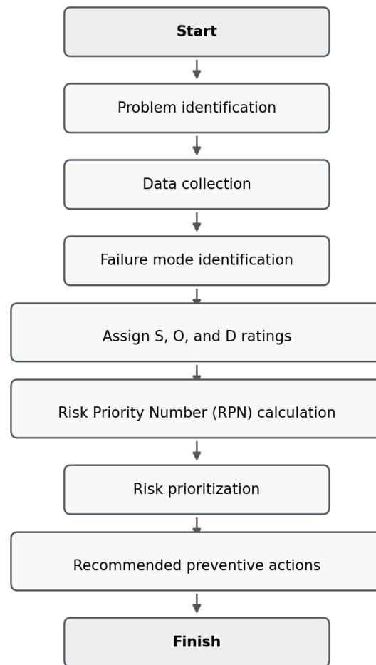
Figure 1. FMEA-Based Screw Press Failure Assessment Procedure at PMKS PT SISIRAU
