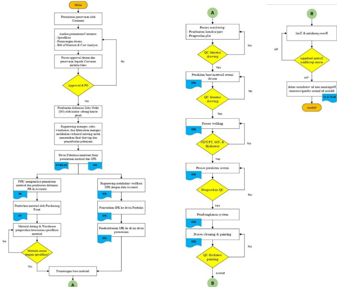
Gambar 1. Diagram alir Proses Produksi Medical System Vacuum
